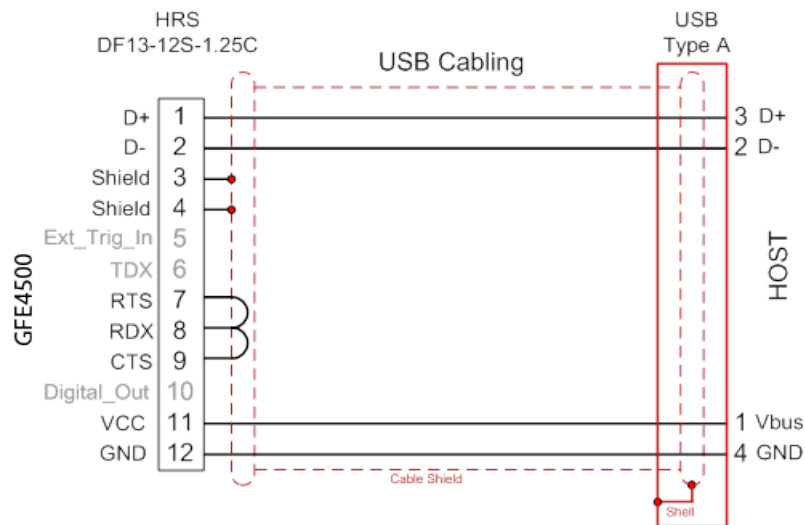
Figure 3. USB cabling
