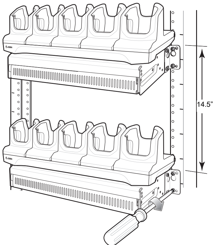
Figure 45 Secure Bracket to Rack (Horizontal Position Shown)
