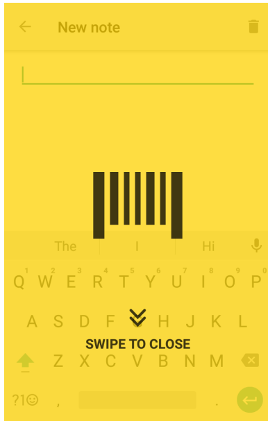
Figure 61 Maximized DCP
