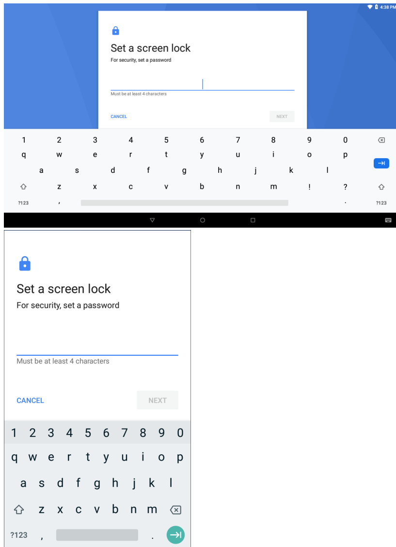
Figure 80 Password Screen
