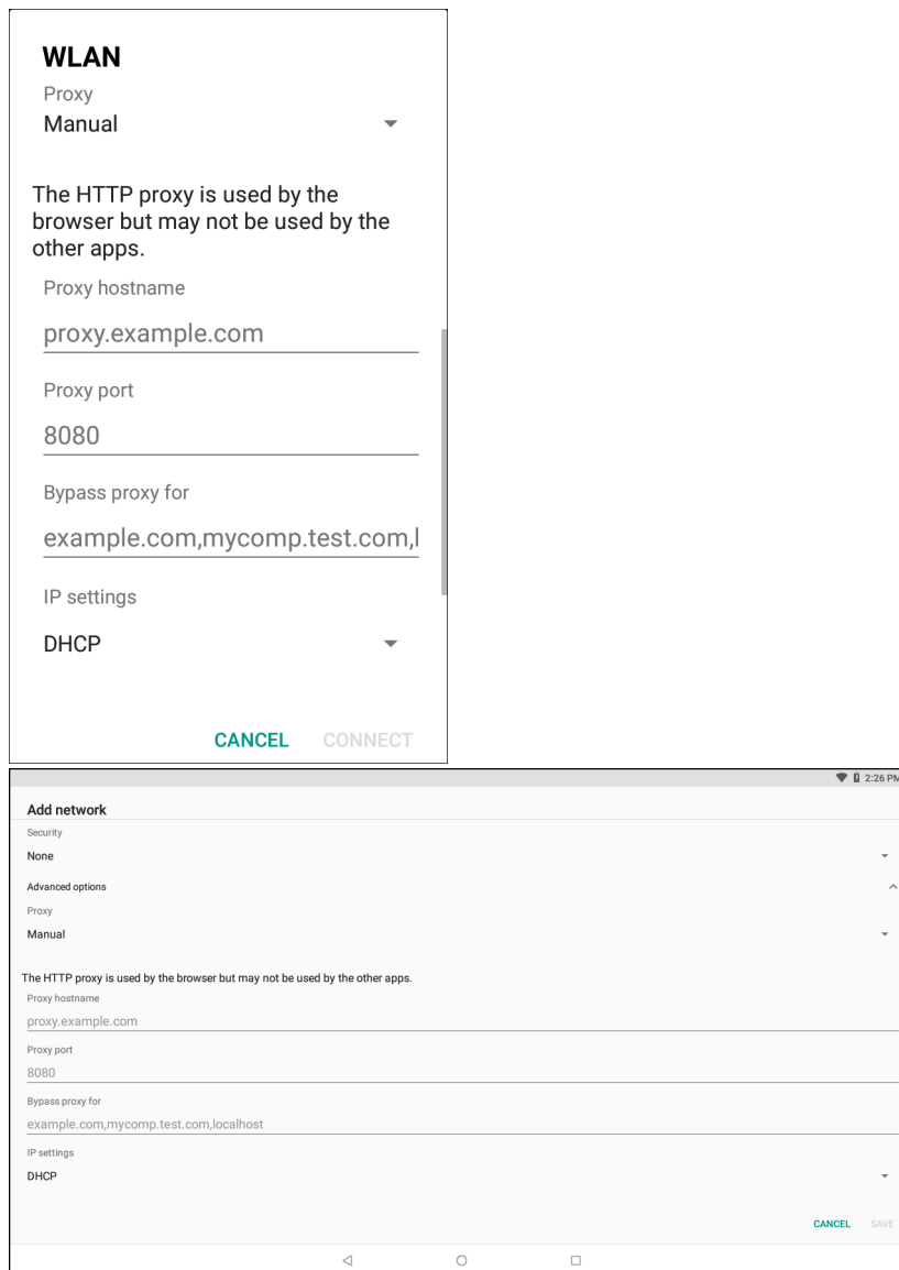
Figure 77 Proxy Settings
