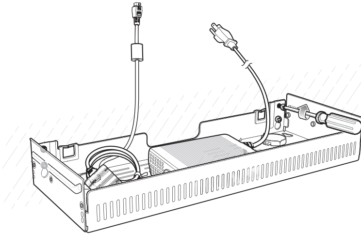
Figure 48 Horizontal Installation - Tighten Screws
