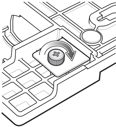
Figure 25 Secure Screw
