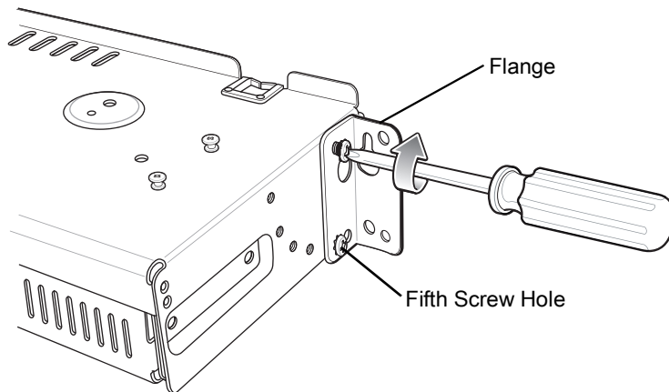
Figure 43 Flange 25° Position
