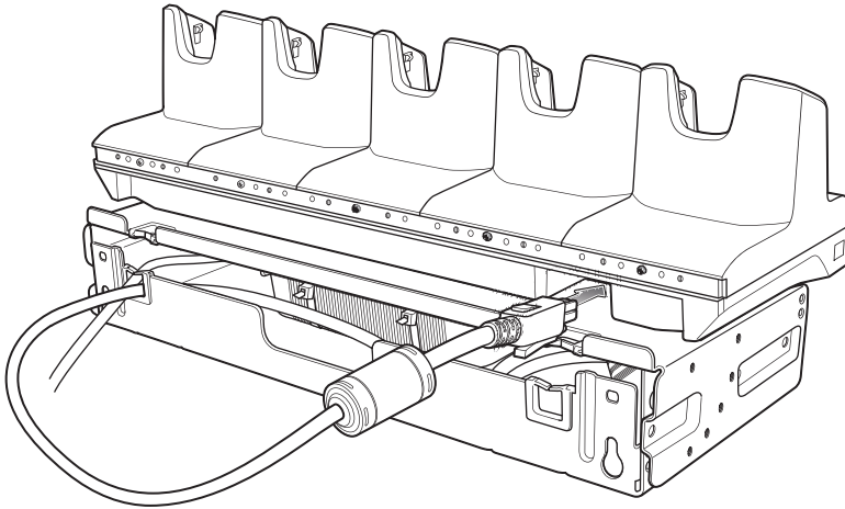
Figure 40 Connect Cables
