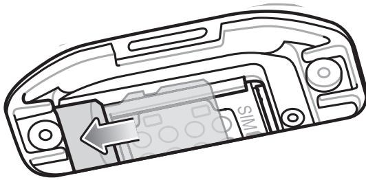
Figure 12 Push microSD Card into the SD Card Slot
