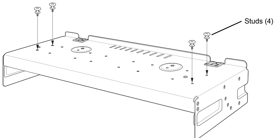
Figure 36 Install Studs
