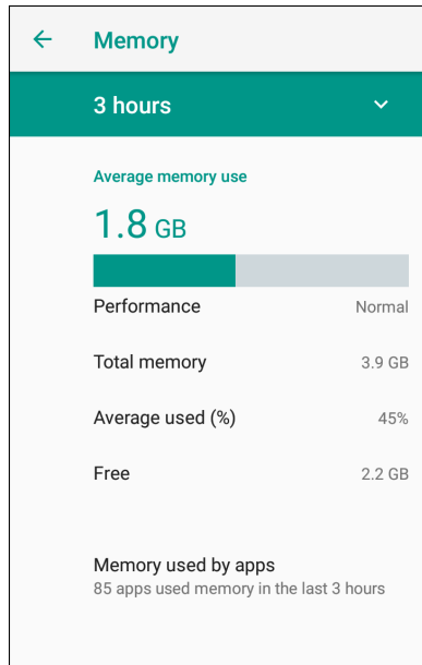
Figure 100 Memory Screen
