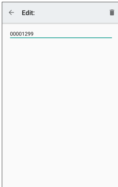
Figure 73 Formatted Data
