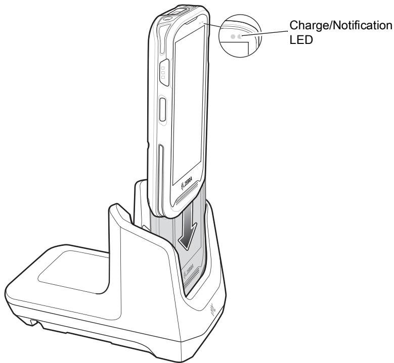
Figure 18 Battery Charging
