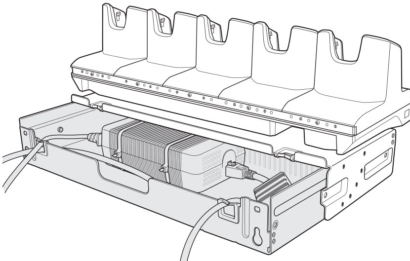
Figure 39 Slide Top Tray onto Bottom Tray
