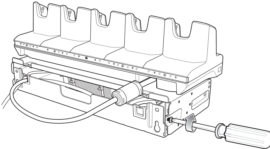
Figure 41 Secure Top and Bottom Tray
