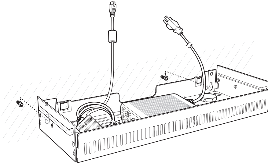
Figure 46 Horizontal Mounting Template
