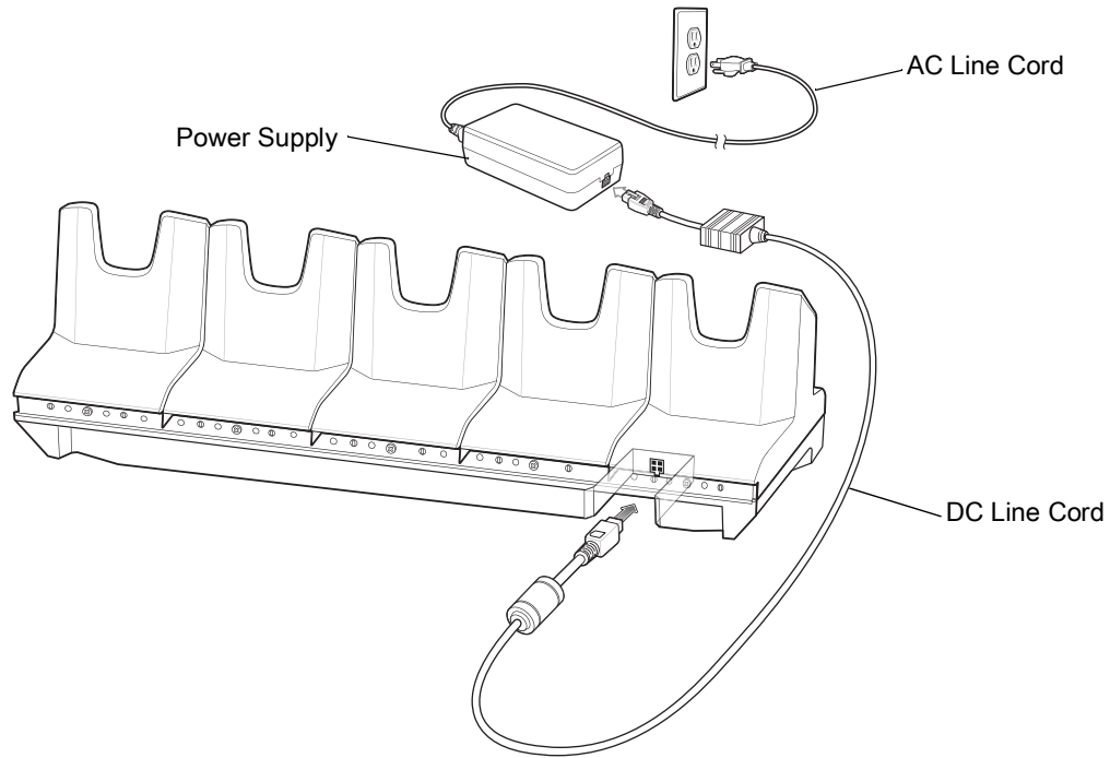
Figure 33 5-Slot Charge Only Cradle Setup
