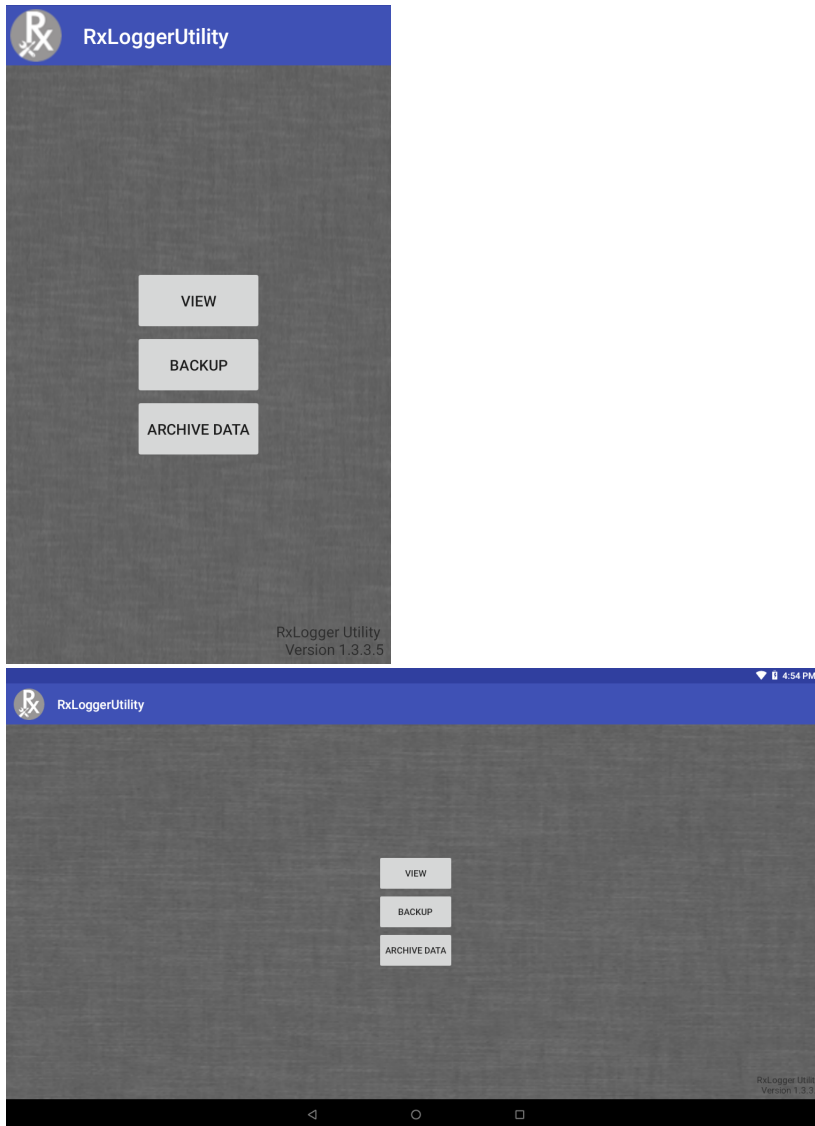
Figure 87 App View
