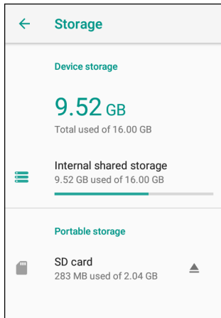
Figure 101 Storage Screen
