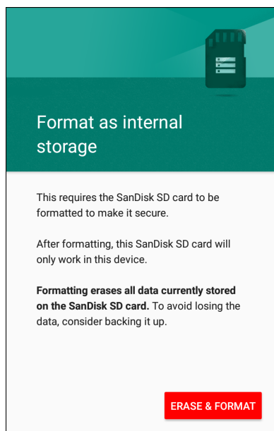
Figure 107 Format Screen
