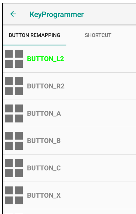
Figure 84 KeyProgrammer Screen
