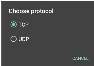
Figure 63 Protocol Selection
