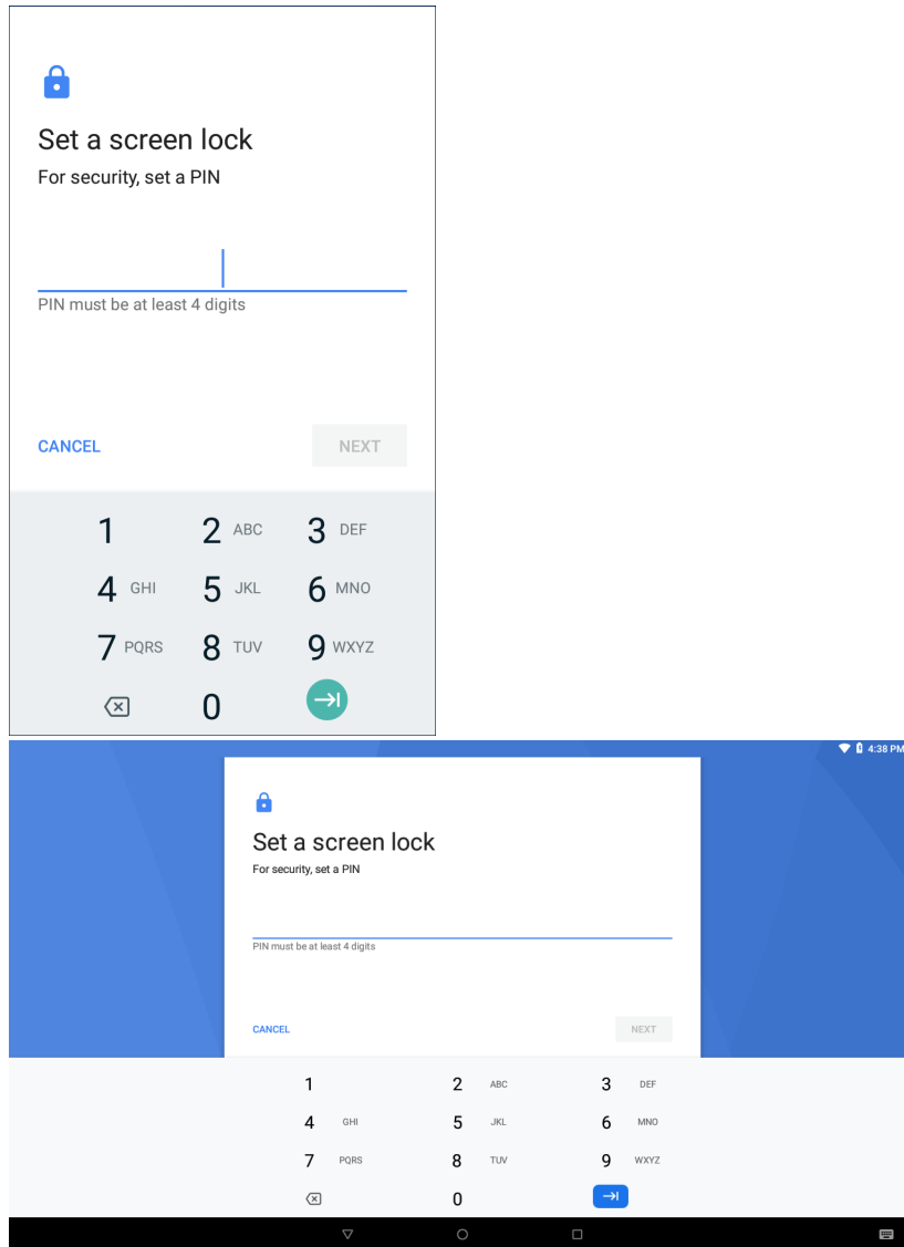
Figure 79 PIN Screen
