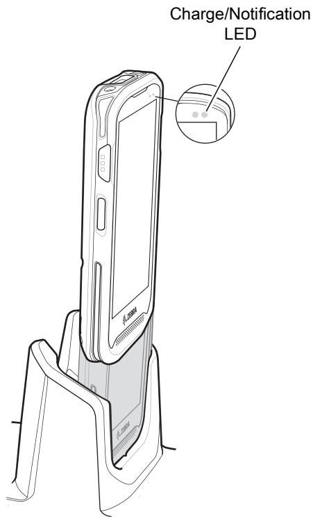
Figure 34 TC20 Battery Charging
