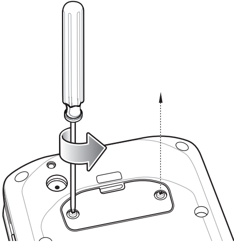
Figure 9 Remove Access Door
