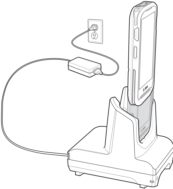
Figure 7 Charging with Cradle
