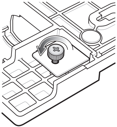
Figure 20 Remove Thumbscrew
