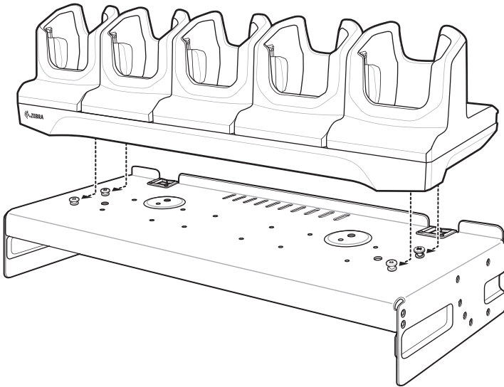
Figure 37 Align Cradle on Studs
