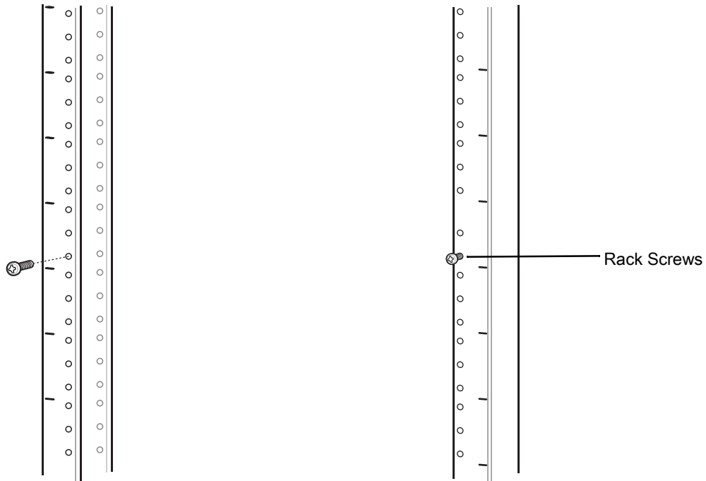
Figure 44 Install Rack System Screws
