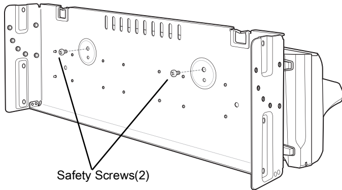
Figure 38 Secure Cradle
