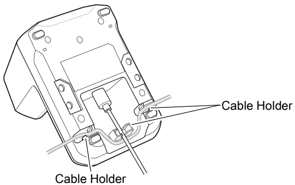
Figure 15 USB Cable Routing
