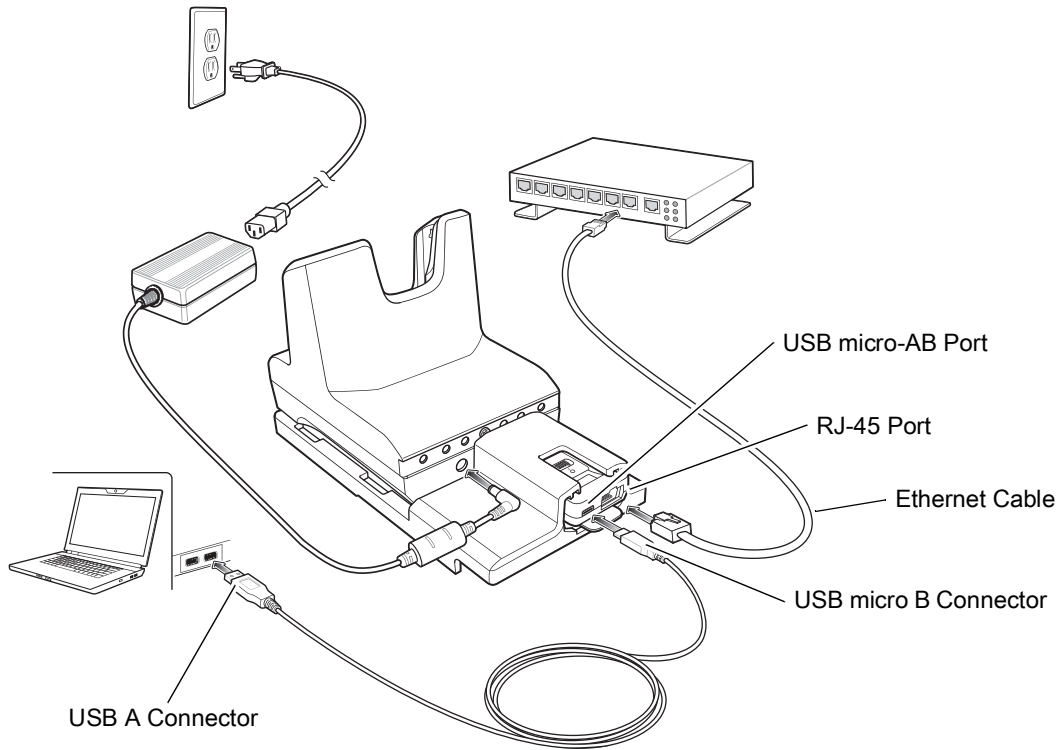
Figure 27 Ethernet Bracket Setup
