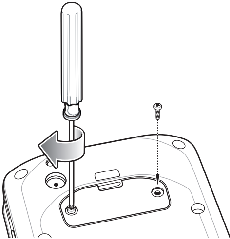
Figure 13 Secure Access Door
