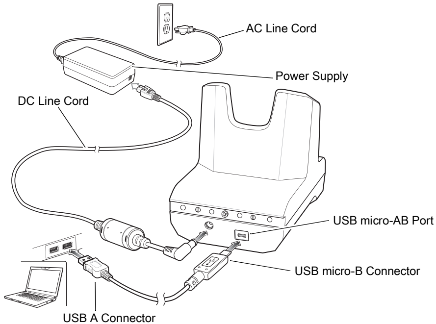
Figure 19 1-Slot USB Charge Cradle Setup
