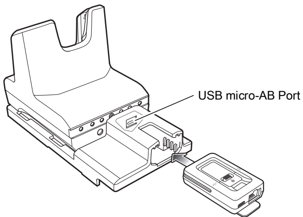
Figure 26 Insert Module
