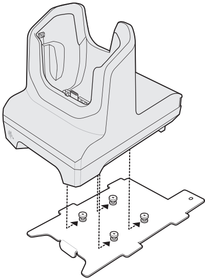
Figure 22 Align Cradle with Plate
