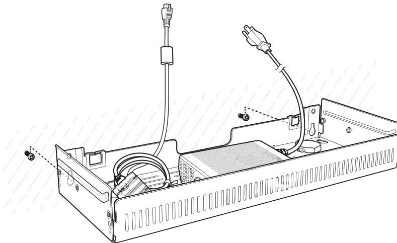
Figure 47 Horizontal Installation
