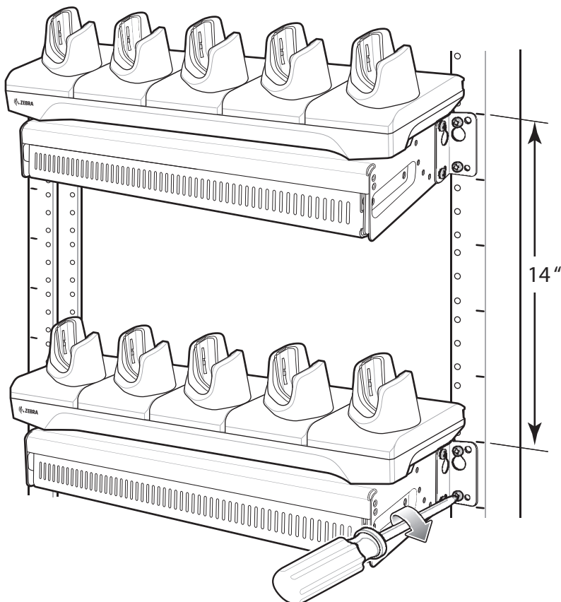
Figure 58 Secure Bracket to Rack (Horizontal Position Shown)
