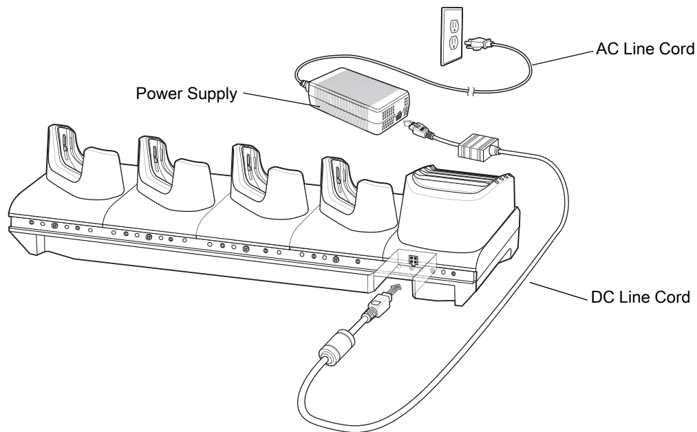
Figure 19 4-Slot Charge Only Cradle with Battery Charger Setup
