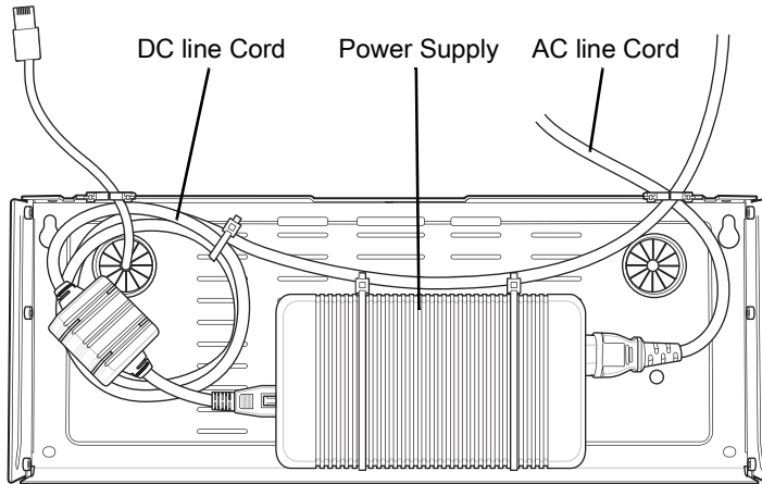
Figure 42 Power Supply in Bottom Tray
