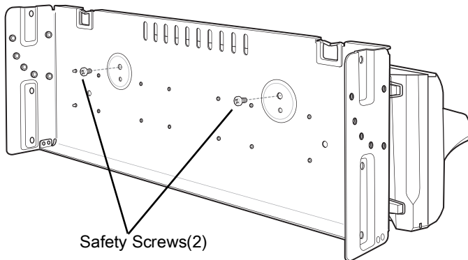
Figure 45 Secure Cradle
