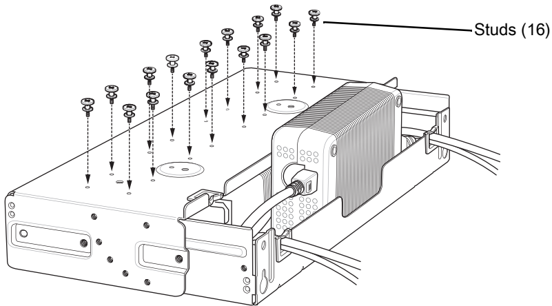
Figure 51 Install Studs
