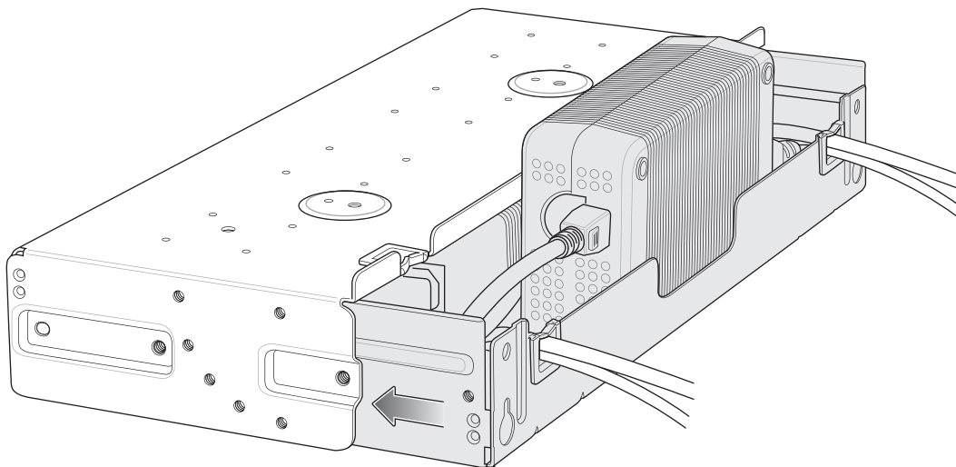
Figure 50 Slide top Tray onto Bottom Tray
