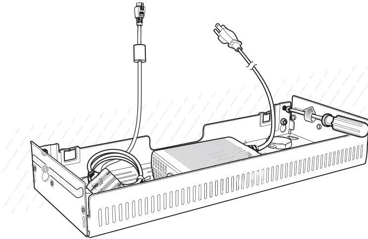
Figure 61 Horizontal Installation - Tighten Screws
