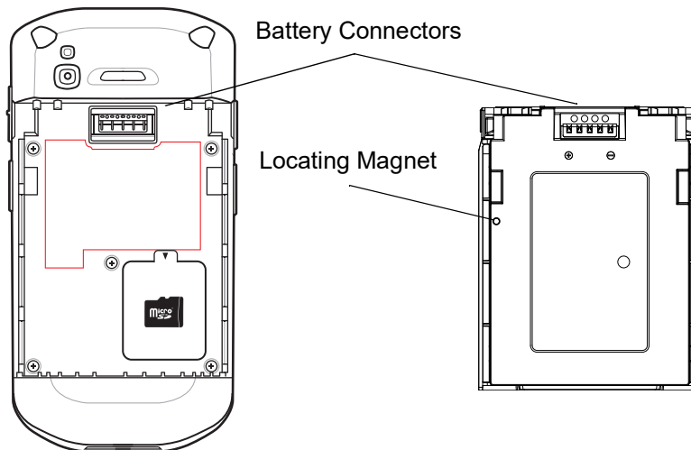
Figure 126 Battery Connectors and Locating Magnet
