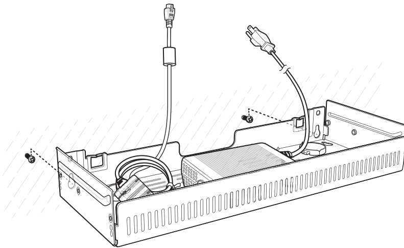
Figure 60 Horizontal Installation
