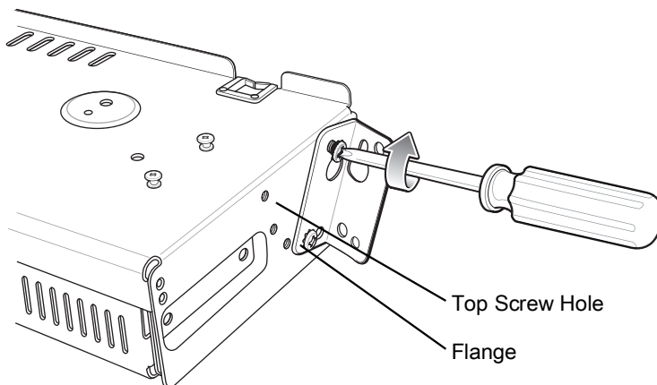
Figure 56 Flange 25° Position (4-Slot Battery Chargers)
