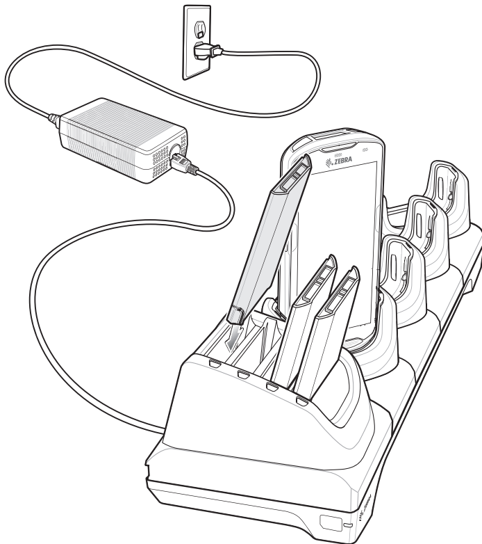
Figure 21 Spare Battery Charging
