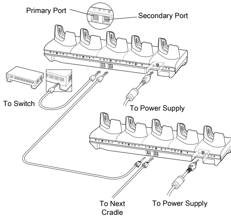
Figure 27 Daisy-chaining 5-Slot Ethernet Cradles
