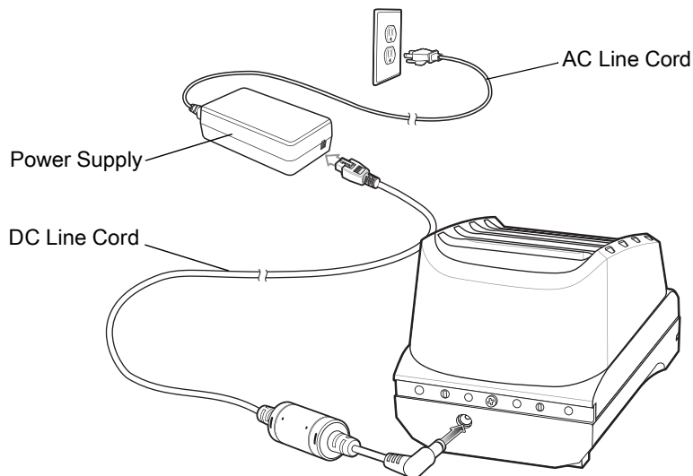
Figure 32 4-Slot Battery Charger Power Setup
