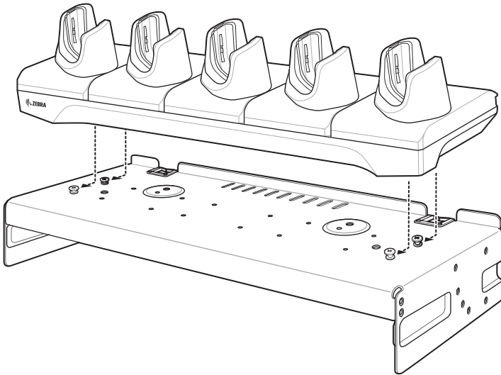
Figure 44 Align Cradle on Studs
