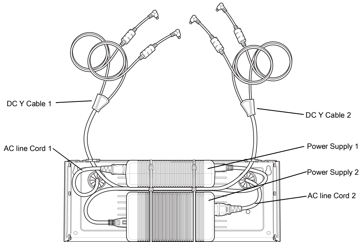
Figure 49 Power Supplies in Bottom Tray
