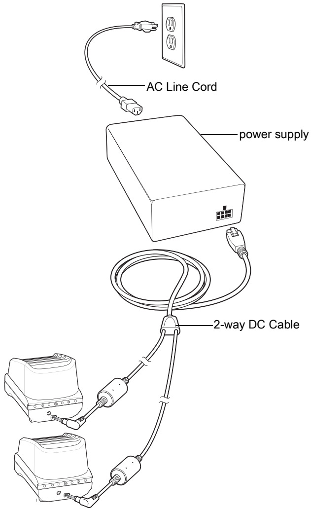
Figure 33 Setup with 2-Way DC Cable
