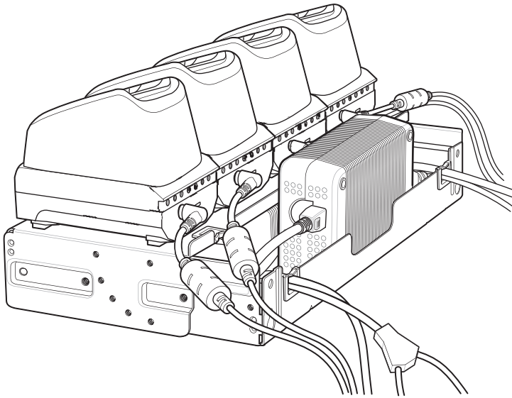
Figure 54 Secure Top Tray to Bottom Tray
