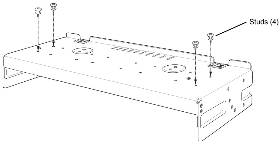
Figure 43 Install Studs
