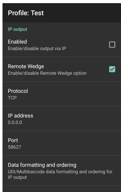
Figure 74 IP Output Screen
