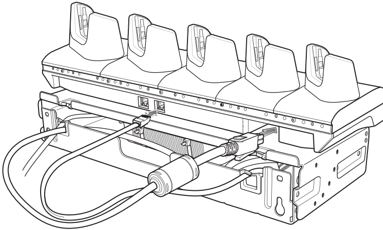
Figure 47 Connect Cables
