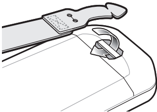
Figure 143 Insert Hand Strap Tab into Slot
