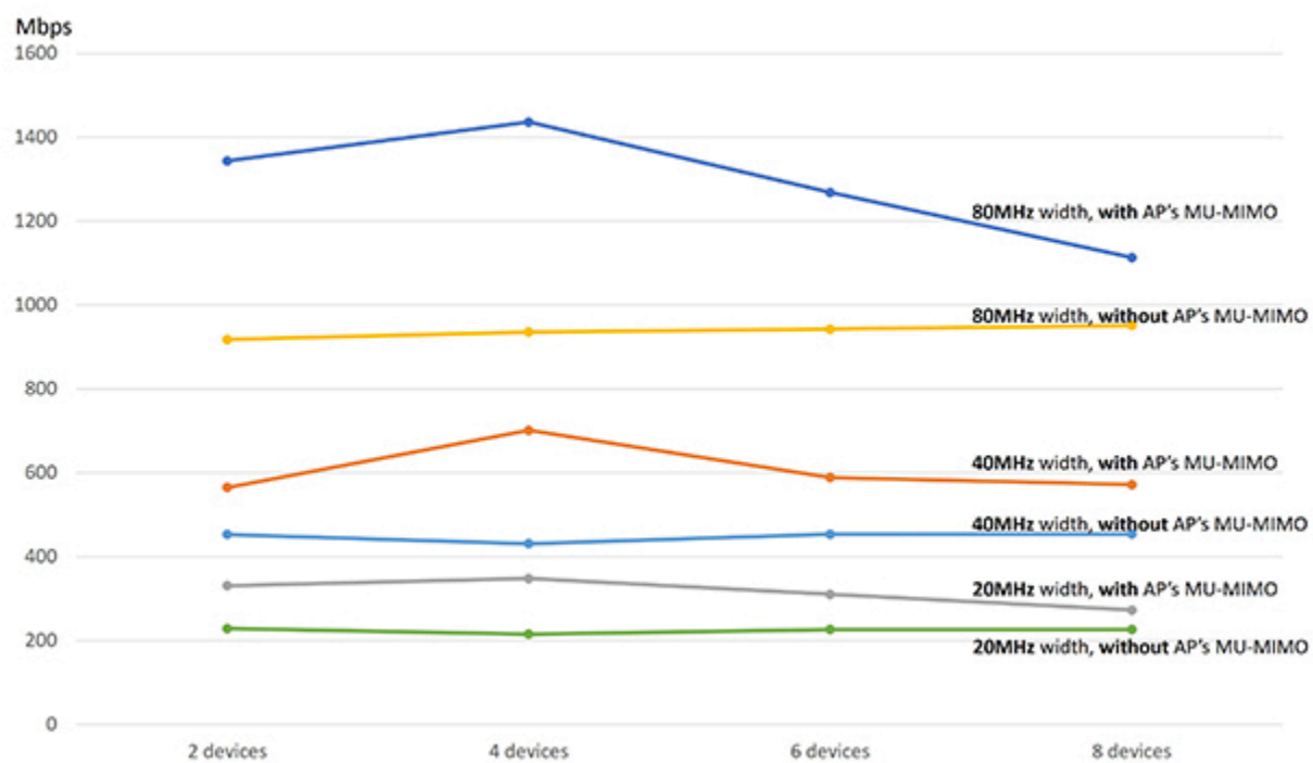
Figure 9 MU-MIMO
