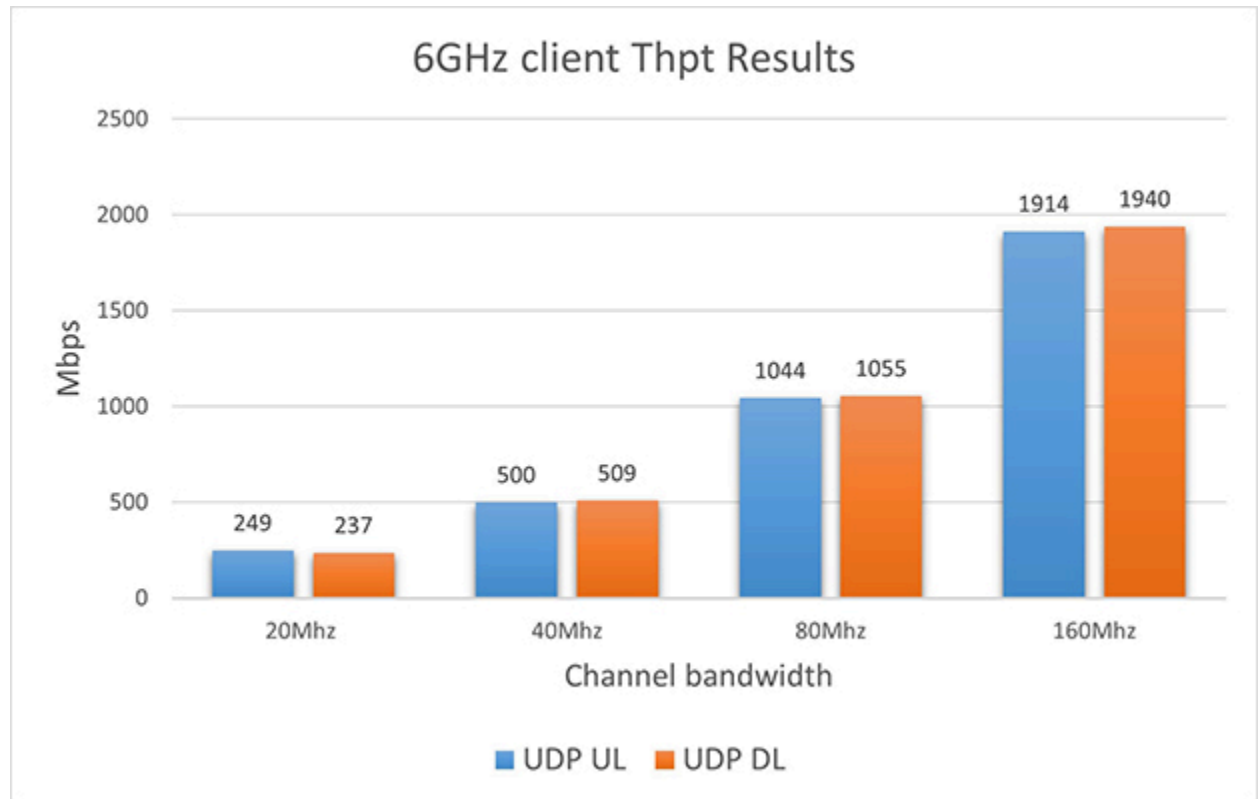
Figure 8 Channel Width for Wi-Fi 6E
