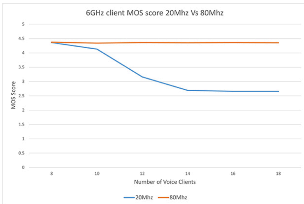
Figure 6 6 GHz Client MOS Score 20 MHz vs 80 MHz
