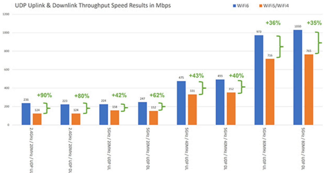
Figure 7 Data Rate Speeds
