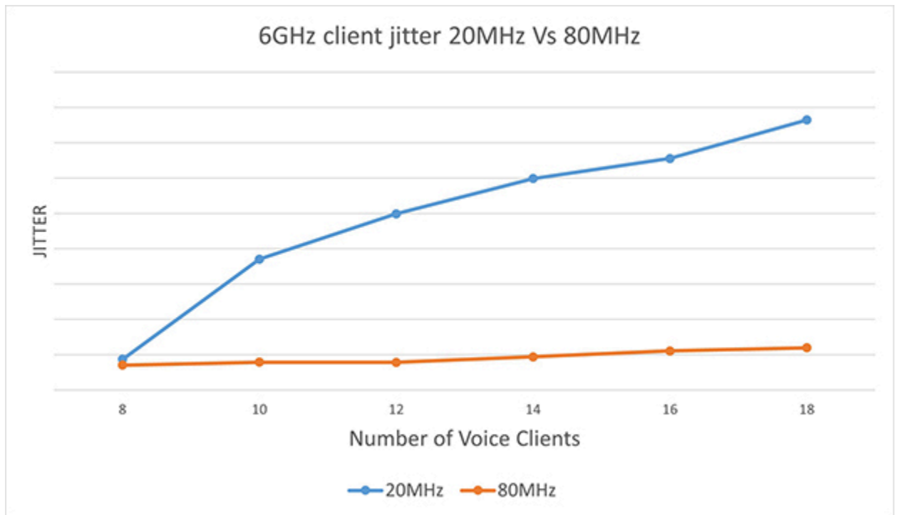
Figure 4 6 GHz Client Jitter 20 MHz vs 80 MHz
